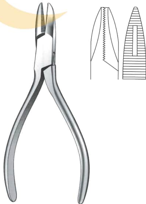
MO-13-991 14 cm / 5 1/2" 2 mm tip Needle nose plier
