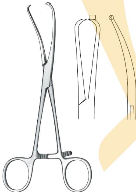
MO-13-775 17 cm / 6¾" Bone holding forceps Curved, with 1.1 mm k-wire guide
